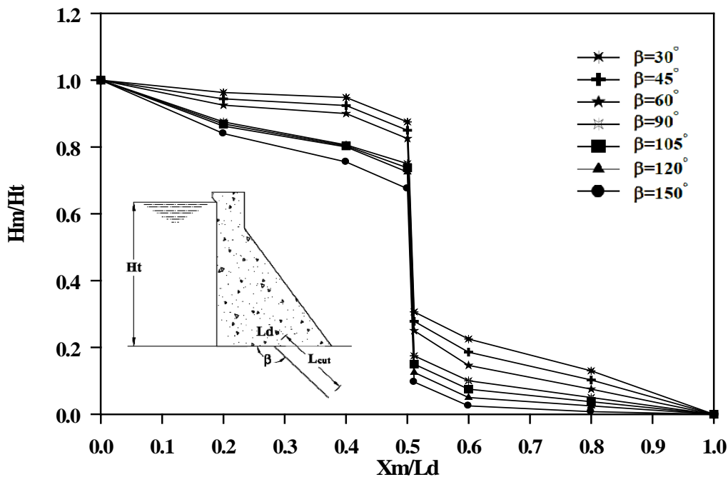
Figure(6): Uplift head ratio through dam foundation vs. a range of ( \beta ) values for cutoff in mid base part of dam
