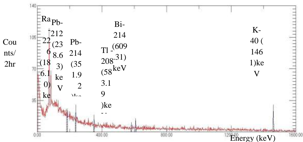
Figure 4. Gamma-rays spectrum for sample (B8).
