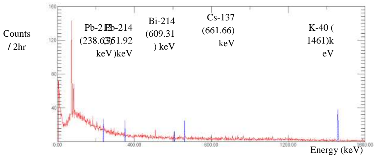
Figure 2. Gamma-rays spectrum for sample (B1).
