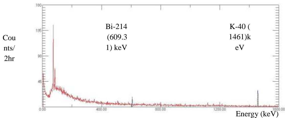
Figure 3. Gamma-rays spectrum for sample (B7).
