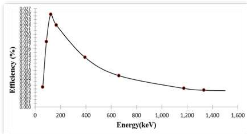
Figure 1. Efficiency calibration curve of (HPGe) detector using standard mixed source.
